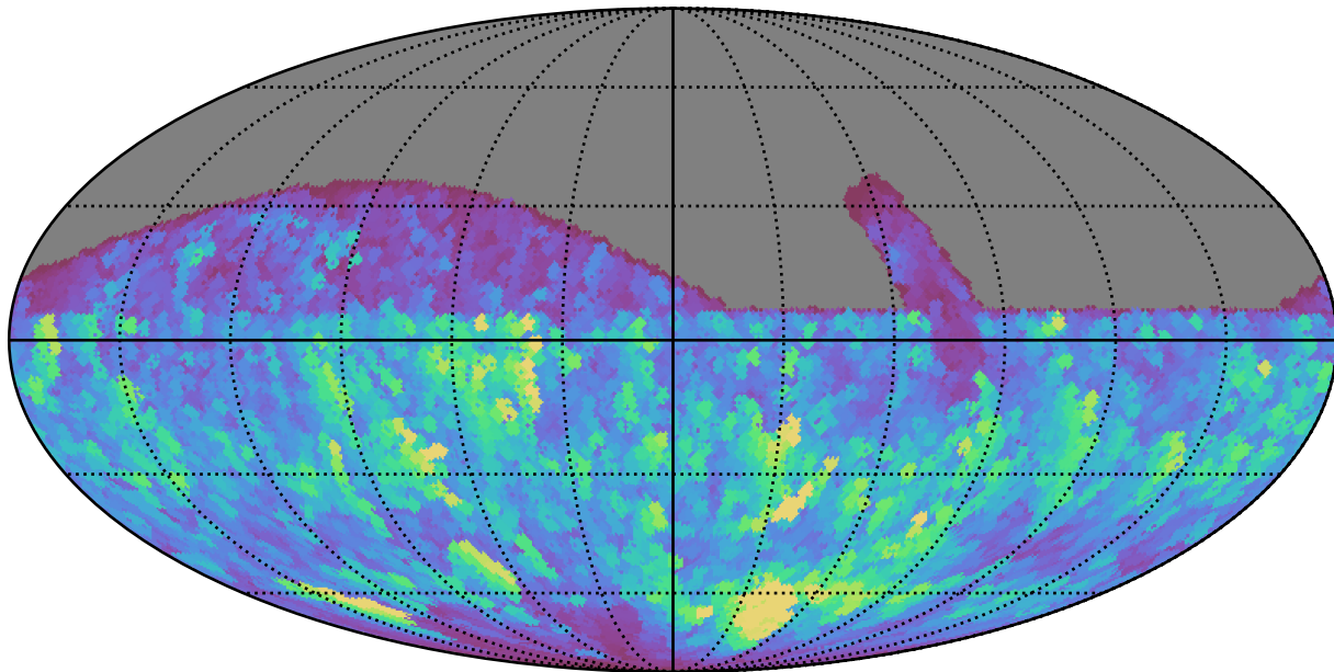
retro_baseline_v2.0_10yrs All sky all bands: Max normairmass
