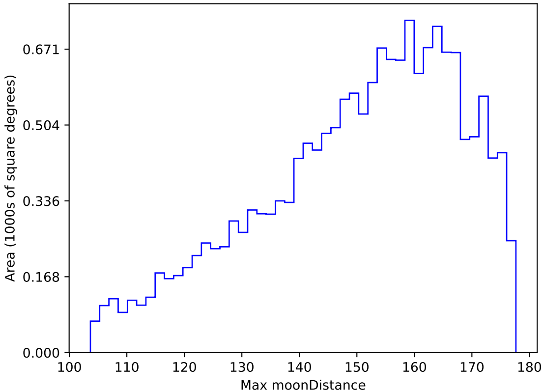
retro_baseline_v2.0_10yrs WFD z band: Max moonDistance
