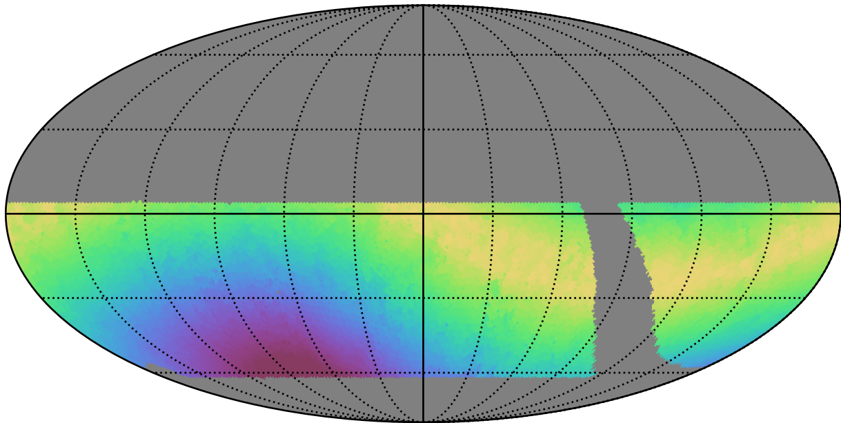
retro_baseline_v2.0_10yrs WFD u band: Max moonDistance
