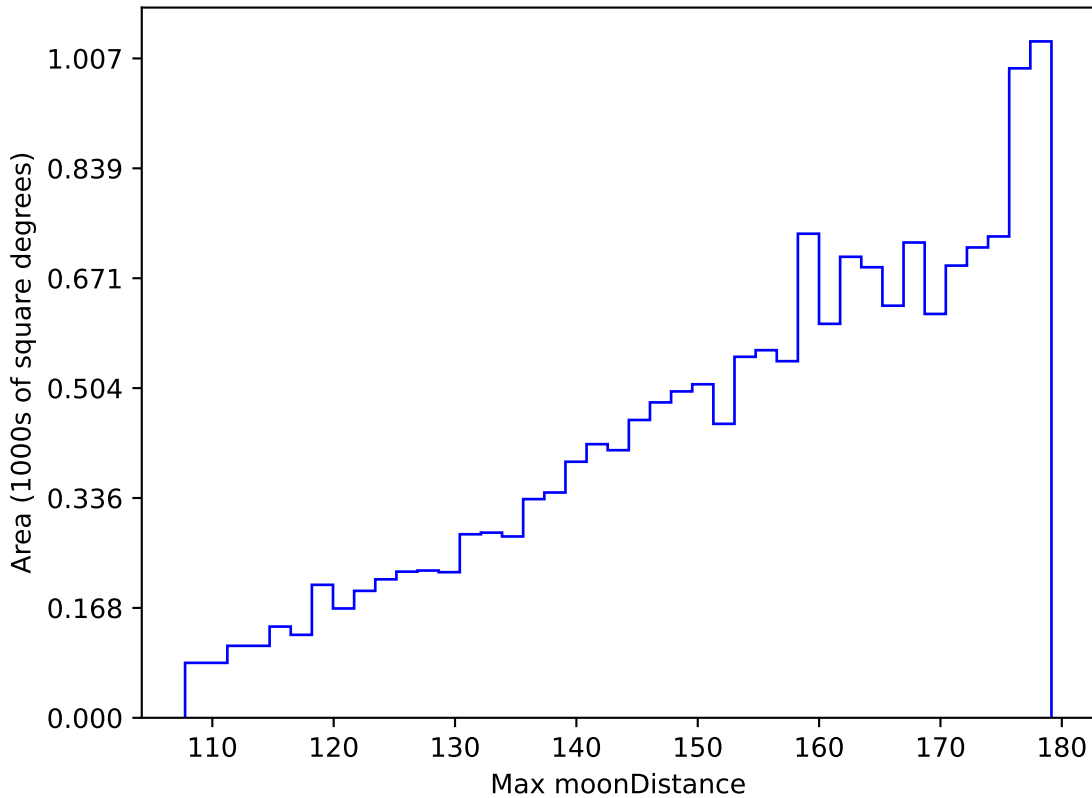
retro_baseline_v2.0_10yrs WFD u band: Max moonDistance
