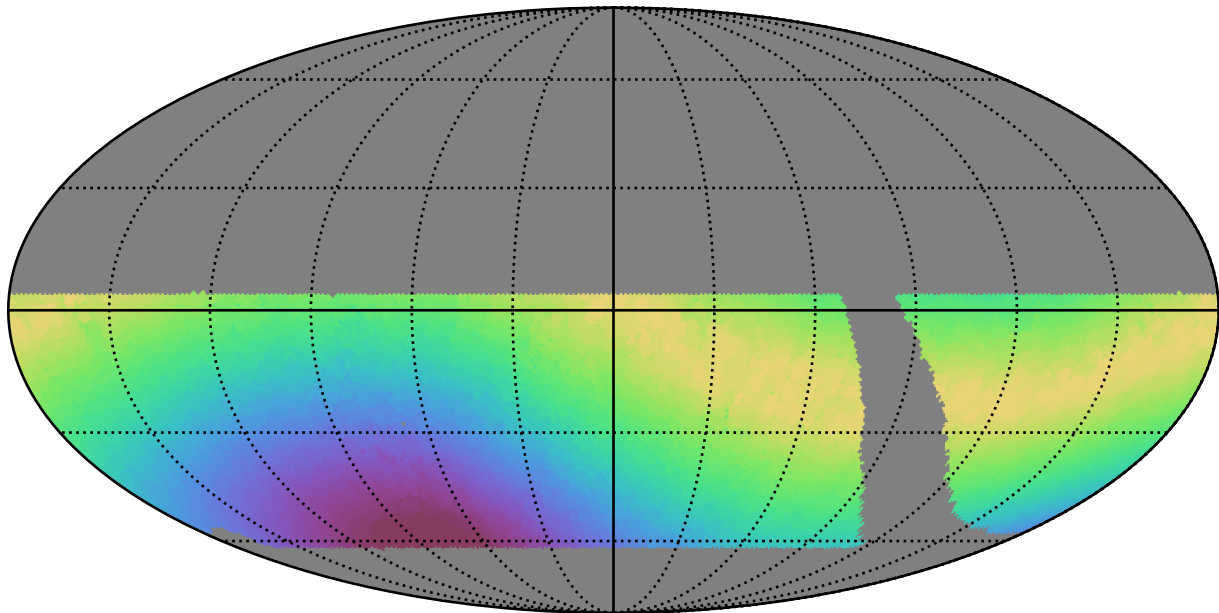
retro_baseline_v2.0_10yrs WFD r band: Max moonDistance
