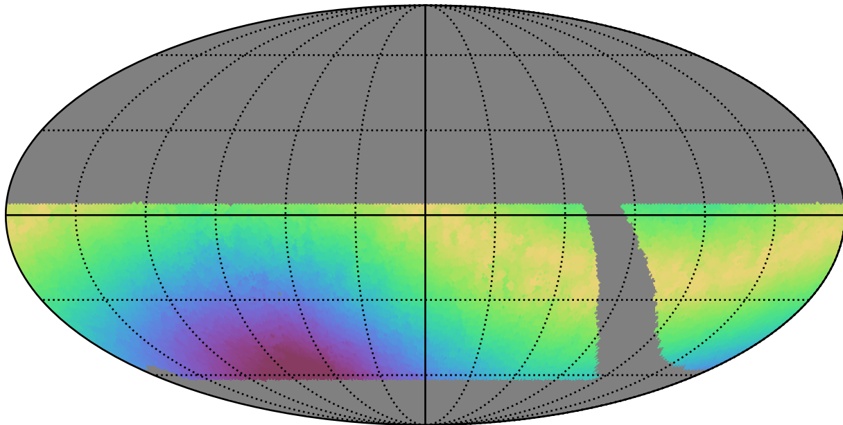
retro_baseline_v2.0_10yrs WFD i band: Max moonDistance
