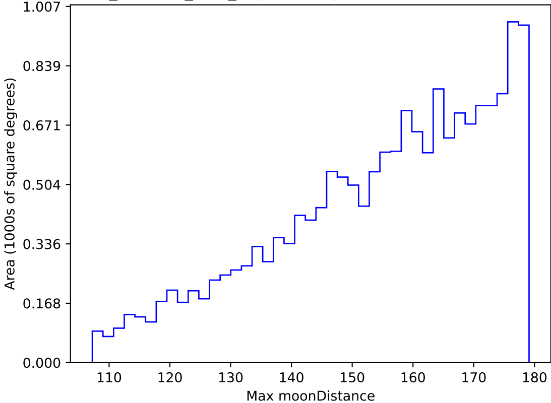
retro_baseline_v2.0_10yrs WFD g band: Max moonDistance
