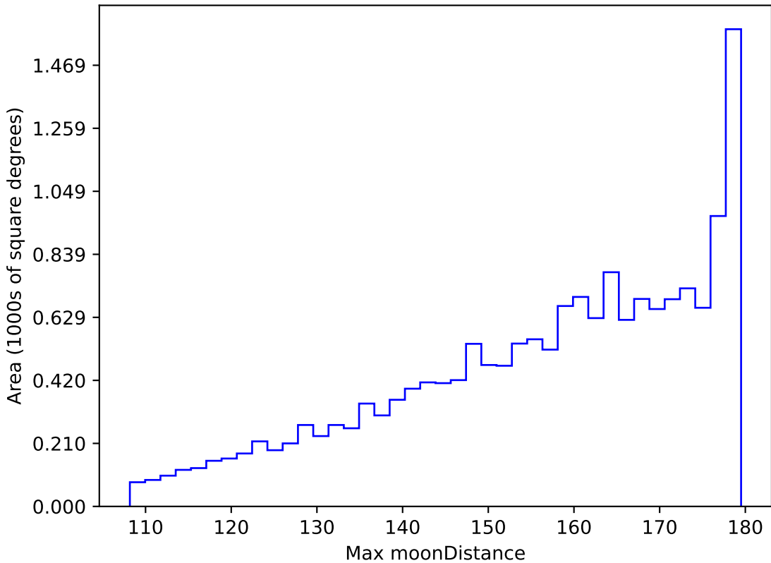
retro_baseline_v2.0_10yrs WFD all bands: Max moonDistance
