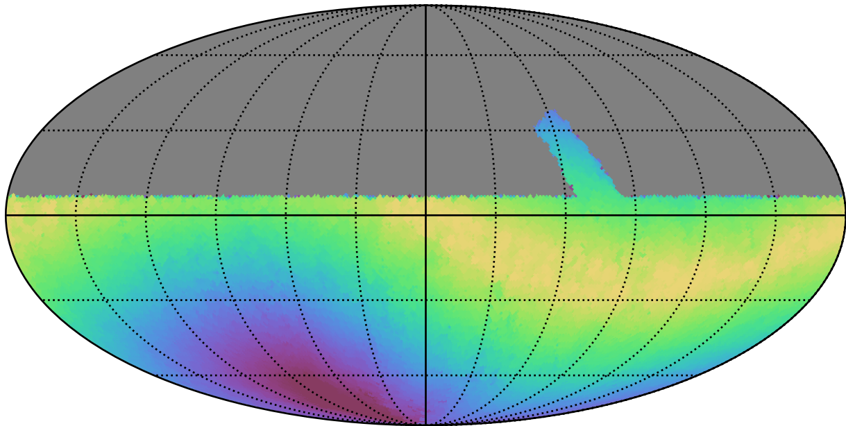
retro_baseline_v2.0_10yrs All sky u band: Max moonDistance
