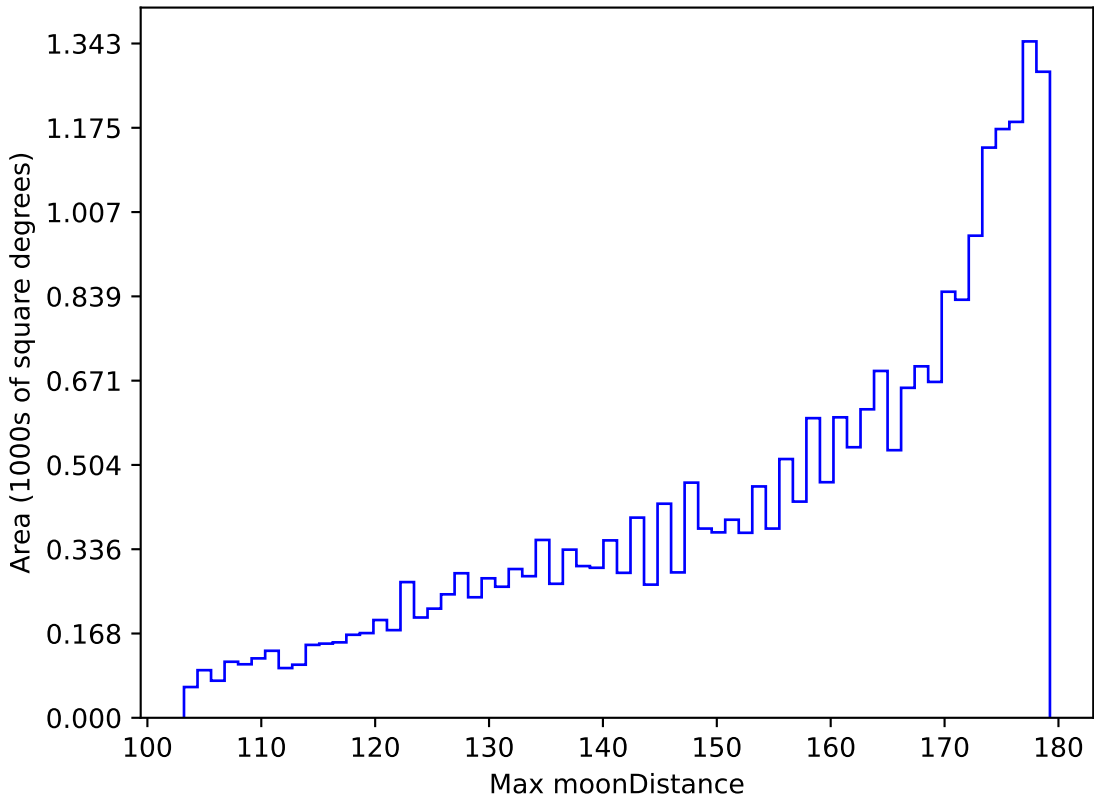
retro_baseline_v2.0_10yrs All sky r band: Max moonDistance
