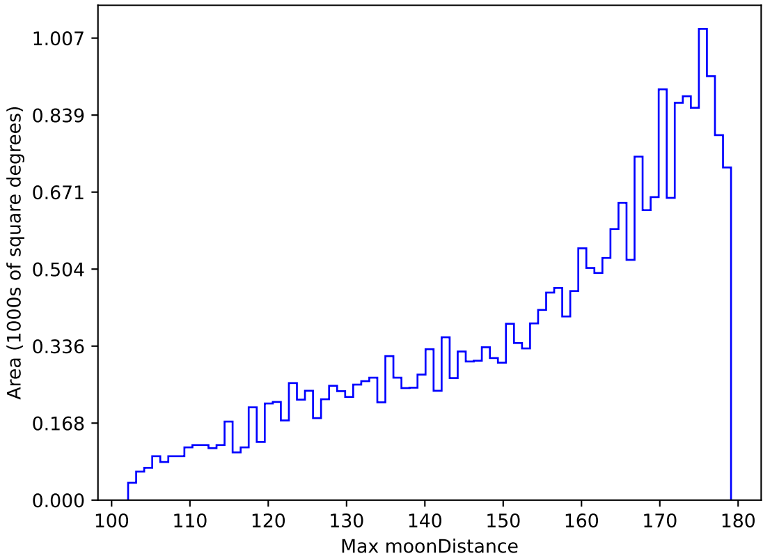
retro_baseline_v2.0_10yrs All sky i band: Max moonDistance
