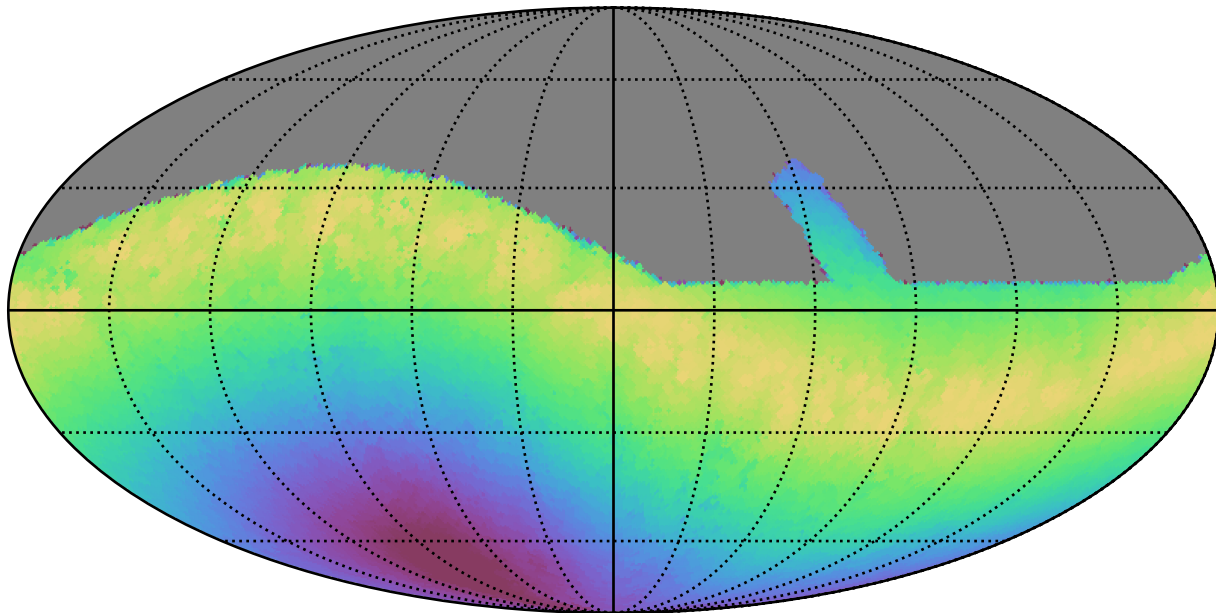
retro_baseline_v2.0_10yrs All sky g band: Max moonDistance
