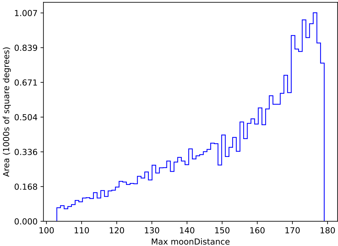
retro_baseline_v2.0_10yrs All sky g band: Max moonDistance
