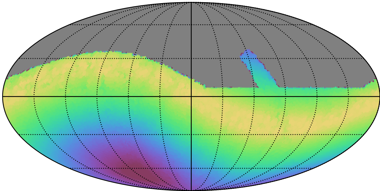
retro_baseline_v2.0_10yrs All sky all bands: Max moonDistance
