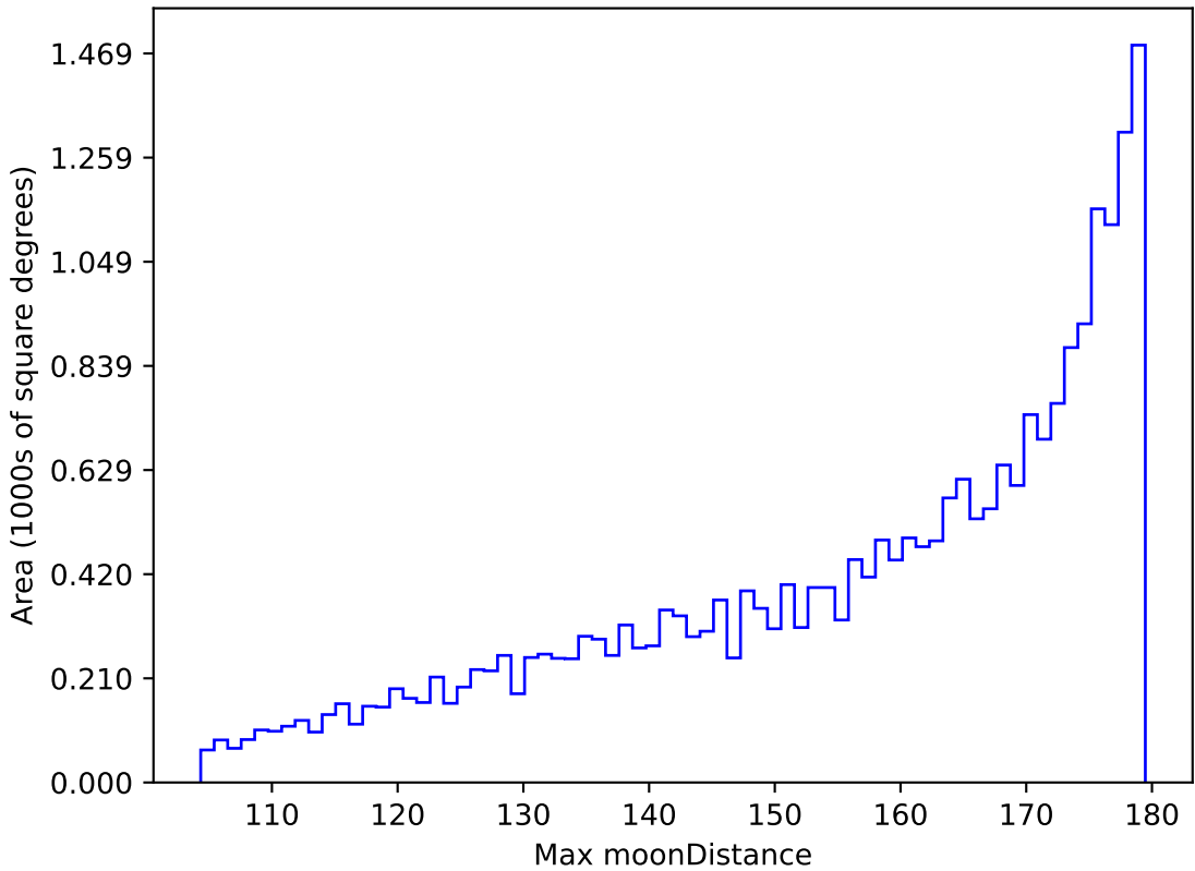
retro_baseline_v2.0_10yrs All sky all bands: Max moonDistance
