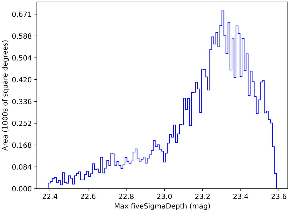
retro_baseline_v2.0_10yrs Yr 1 z band: Max fiveSigmaDepth
