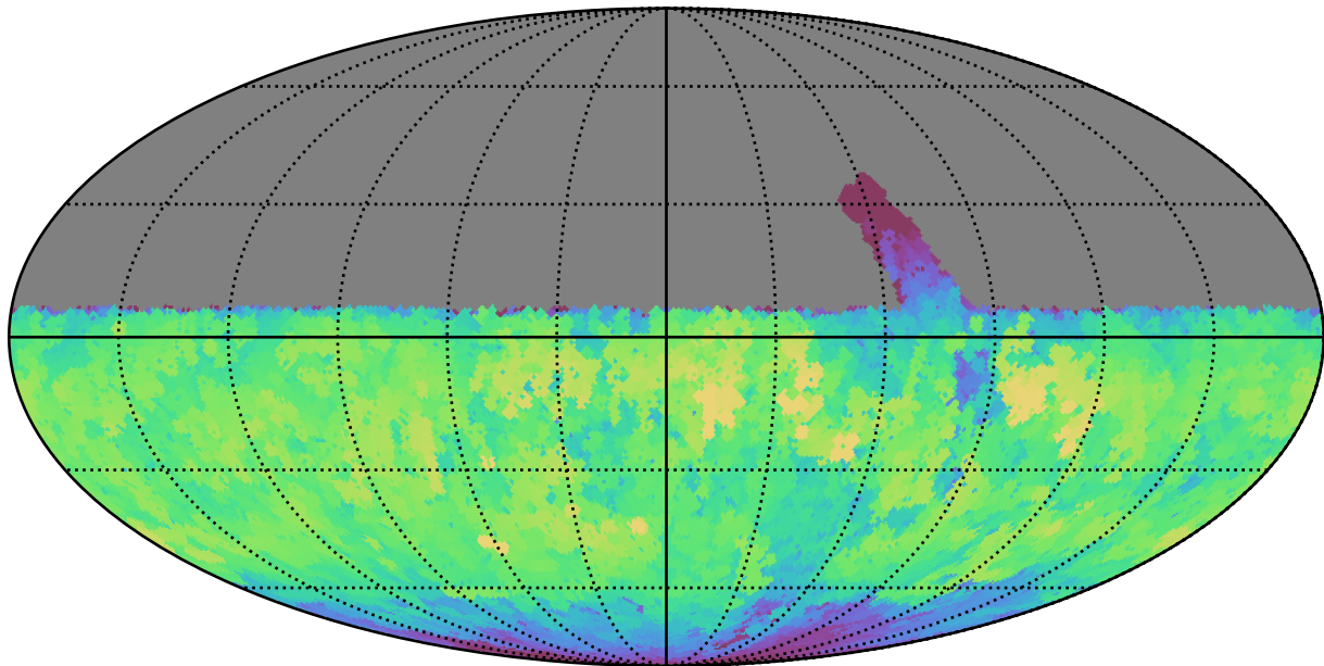
retro_baseline_v2.0_10yrs Yr 1 y band: Max fiveSigmaDepth
