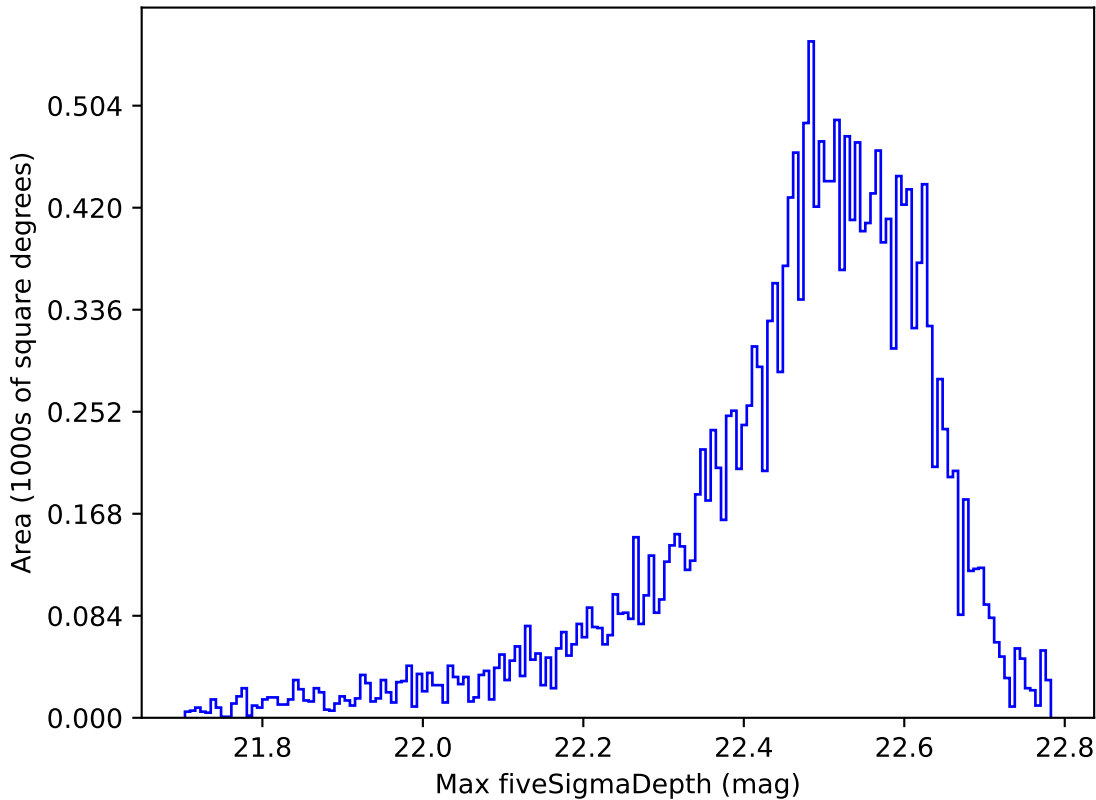
retro_baseline_v2.0_10yrs Yr 1 y band: Max fiveSigmaDepth
