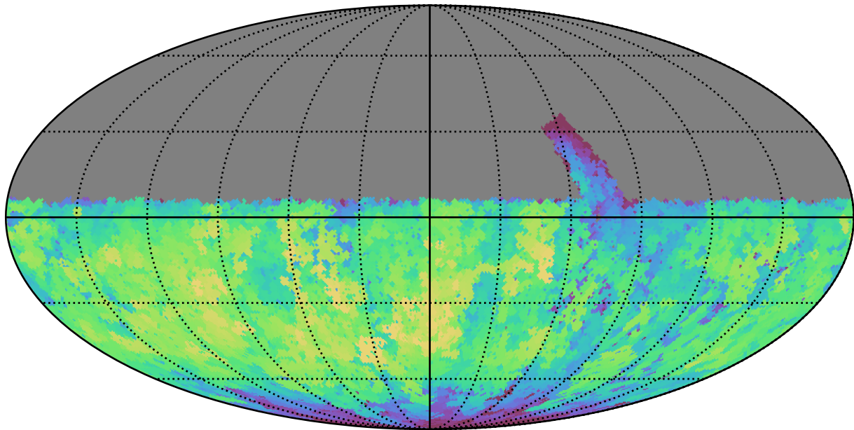
retro_baseline_v2.0_10yrs Yr 1 u band: Max fiveSigmaDepth
