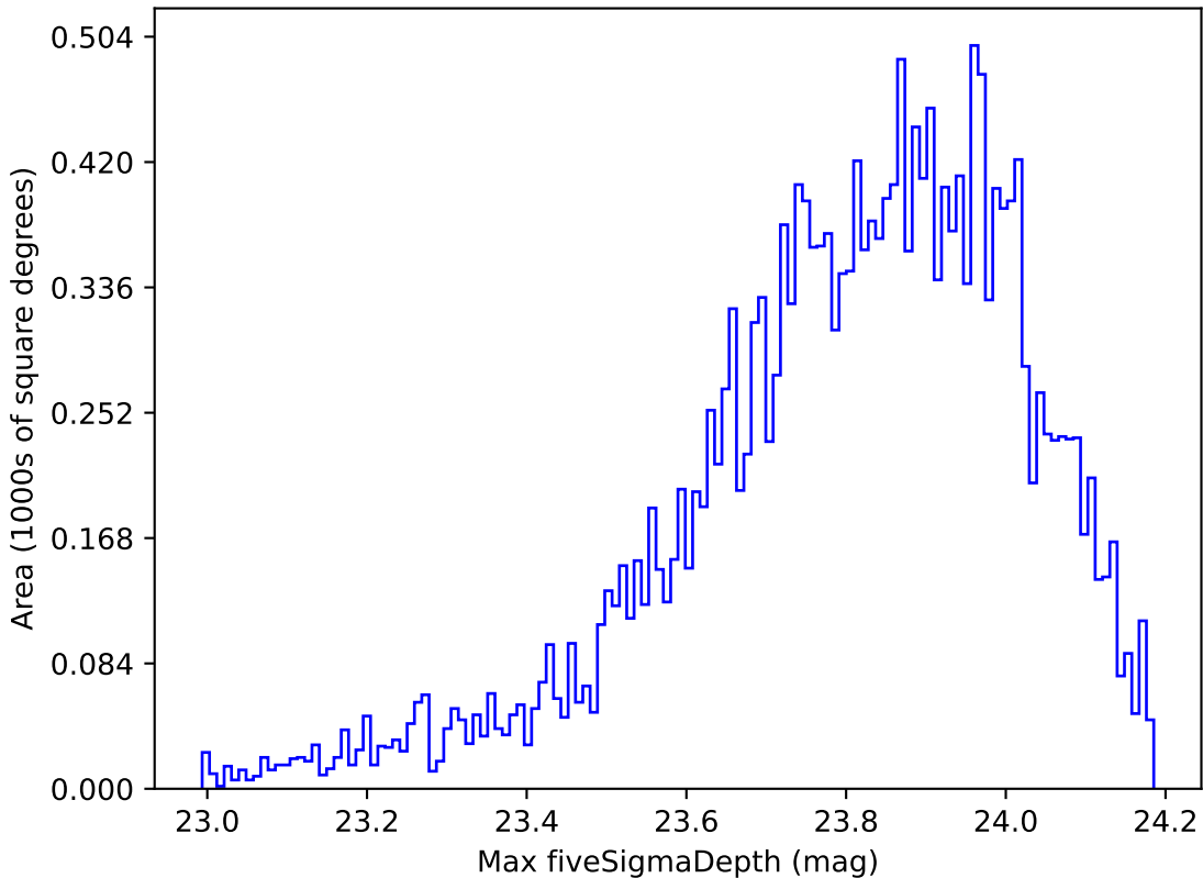
retro_baseline_v2.0_10yrs Yr 1 u band: Max fiveSigmaDepth
