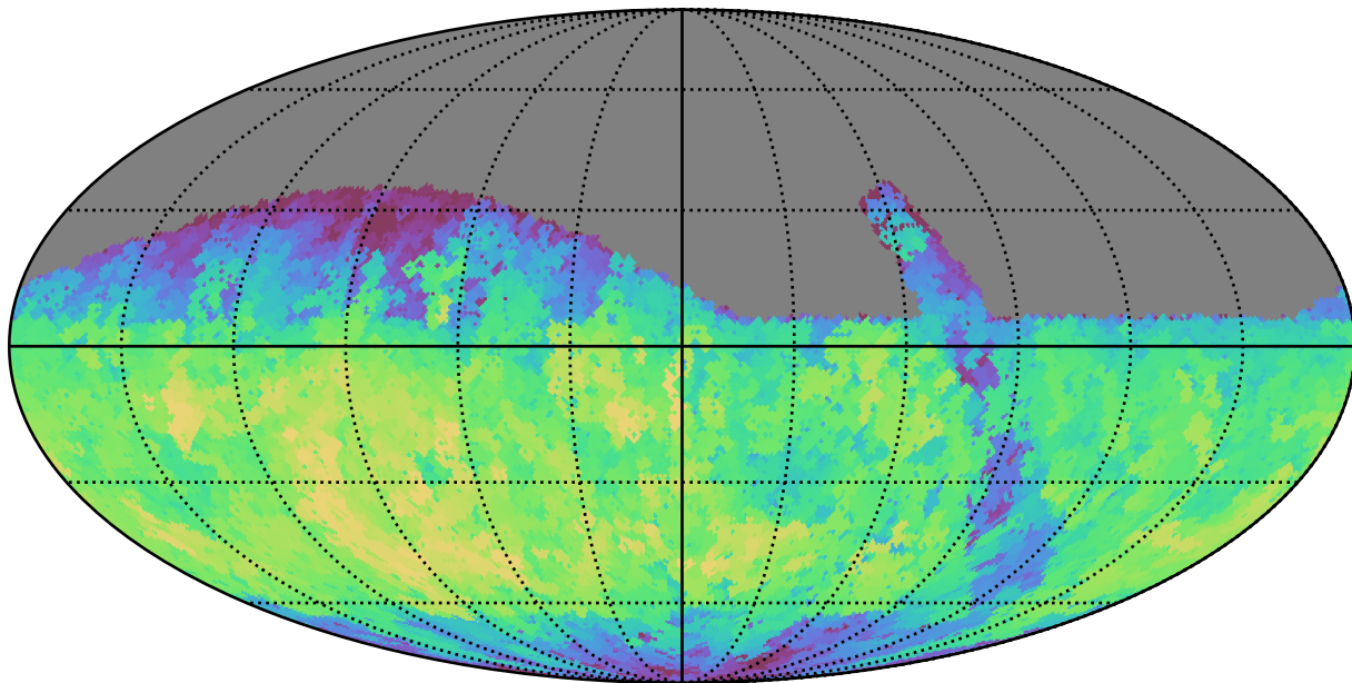
retro_baseline_v2.0_10yrs Yr 1 r band: Max fiveSigmaDepth
