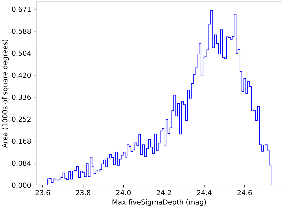
retro_baseline_v2.0_10yrs Yr 1 r band: Max fiveSigmaDepth
