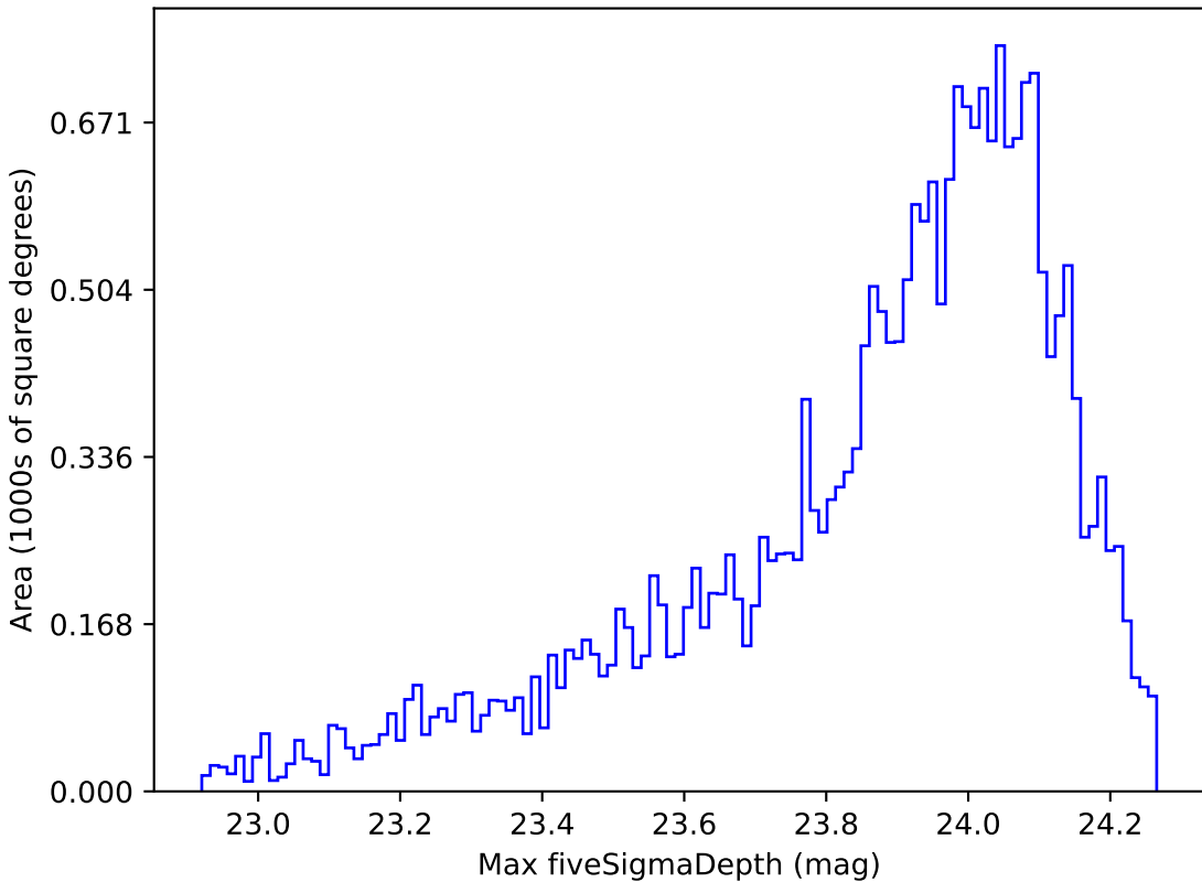
retro_baseline_v2.0_10yrs Yr 1 i band: Max fiveSigmaDepth
