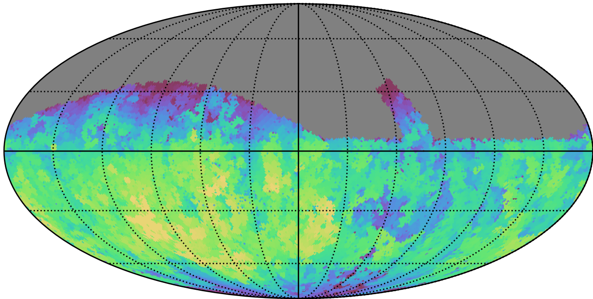
retro_baseline_v2.0_10yrs Yr 1 g band: Max fiveSigmaDepth
