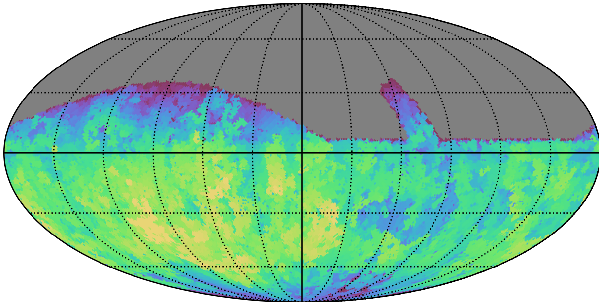
retro_baseline_v2.0_10yrs Yr 1 all bands: Max fiveSigmaDepth
