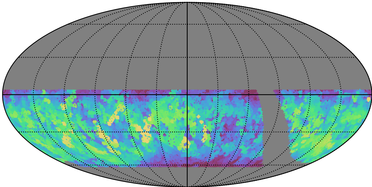
retro_baseline_v2.0_10yrs WFD z band: Max fiveSigmaDepth
