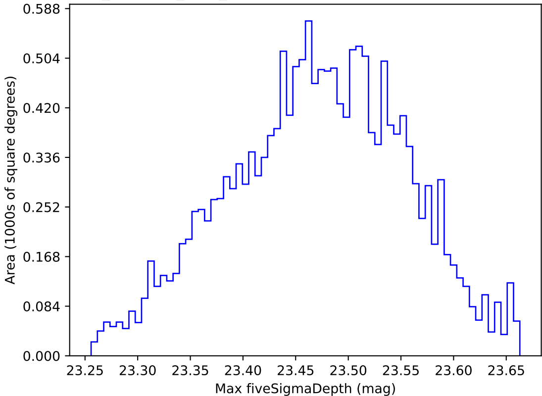
retro_baseline_v2.0_10yrs WFD z band: Max fiveSigmaDepth
