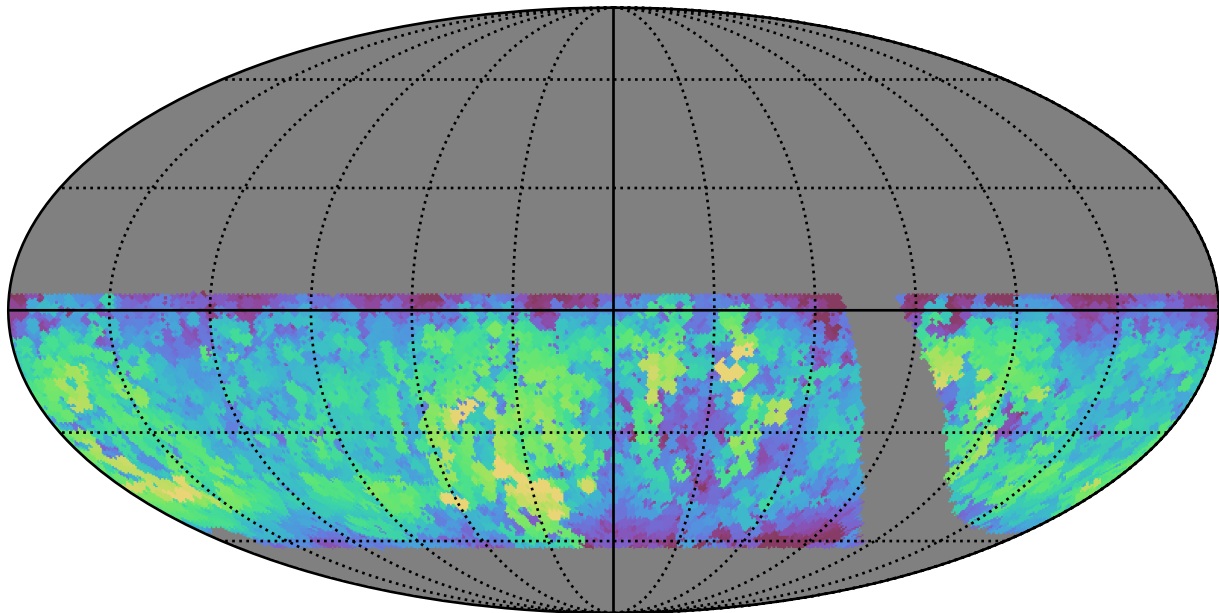
retro_baseline_v2.0_10yrs WFD y band: Max fiveSigmaDepth
