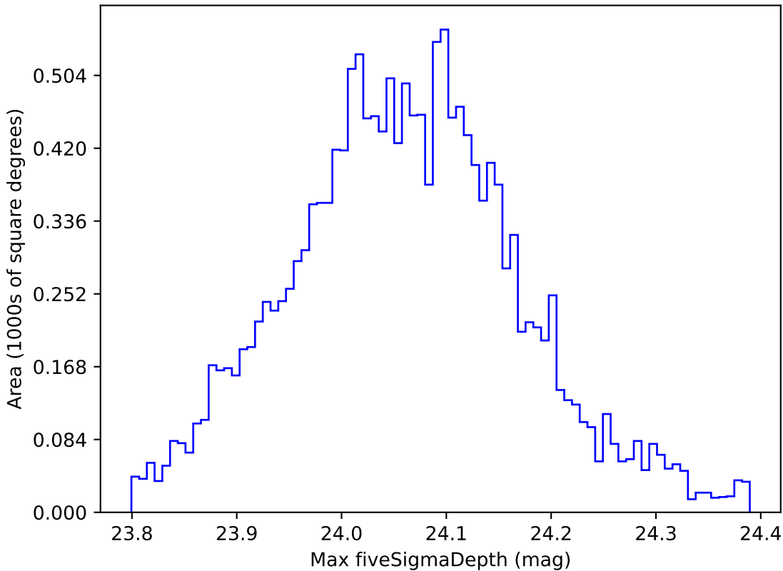
retro_baseline_v2.0_10yrs WFD u band: Max fiveSigmaDepth
