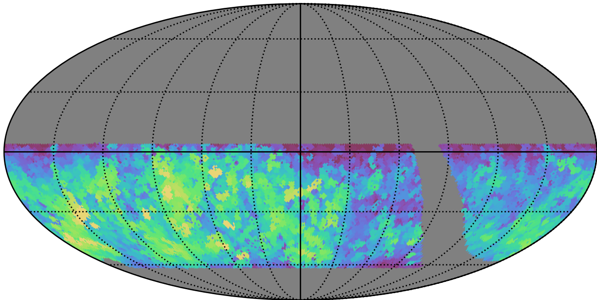
retro_baseline_v2.0_10yrs WFD i band: Max fiveSigmaDepth
