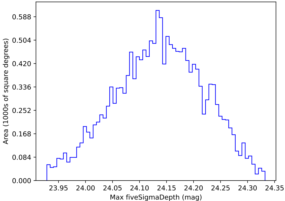
retro_baseline_v2.0_10yrs WFD i band: Max fiveSigmaDepth
