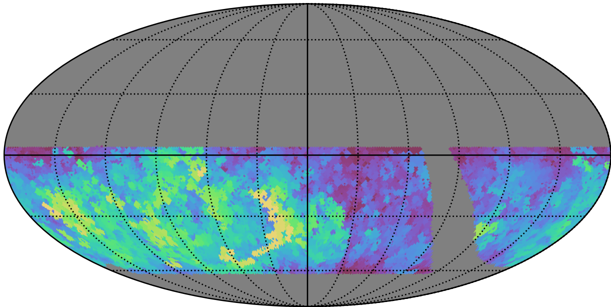
retro_baseline_v2.0_10yrs WFD g band: Max fiveSigmaDepth
