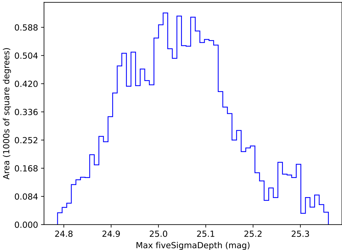
retro_baseline_v2.0_10yrs WFD g band: Max fiveSigmaDepth
