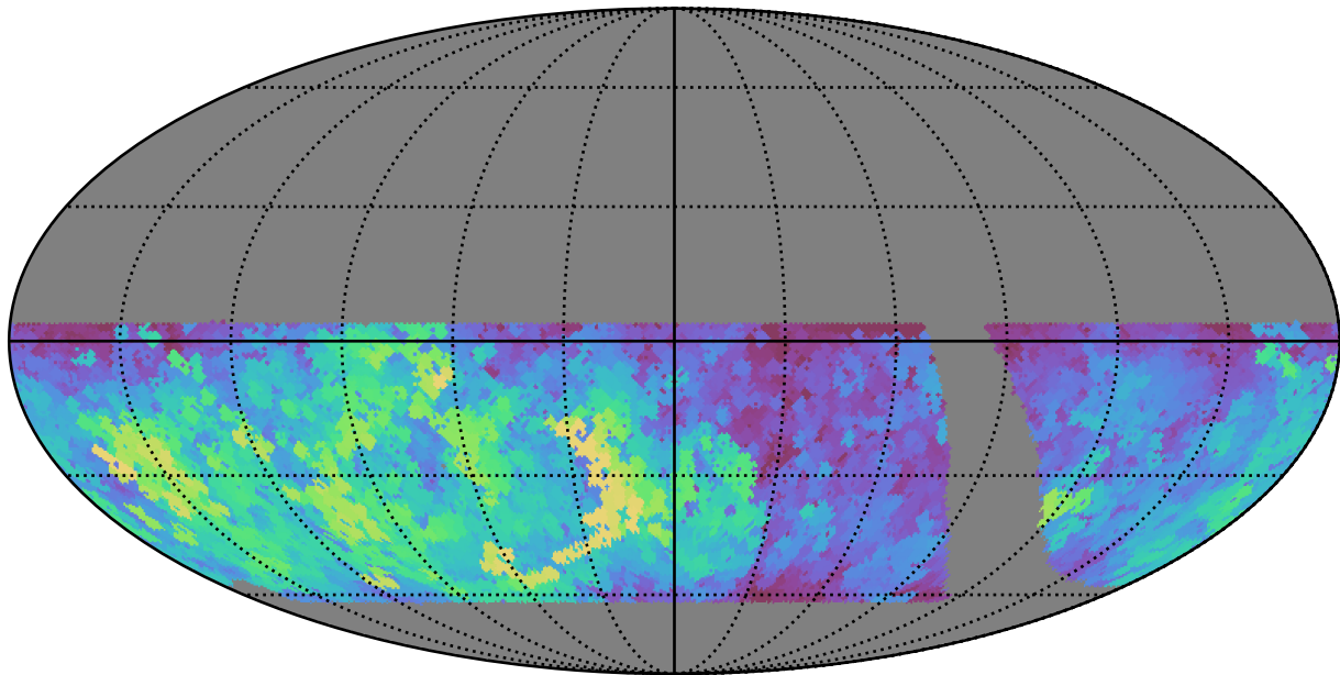
retro_baseline_v2.0_10yrs WFD all bands: Max fiveSigmaDepth
