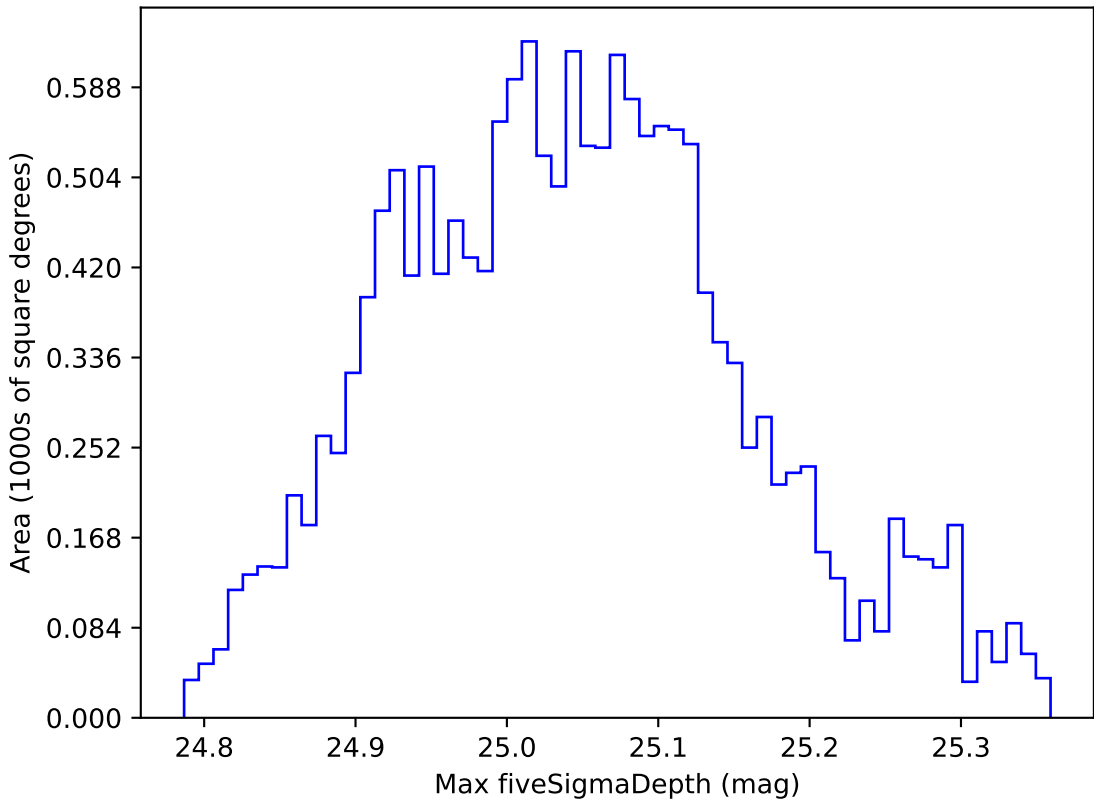
retro_baseline_v2.0_10yrs WFD all bands: Max fiveSigmaDepth
