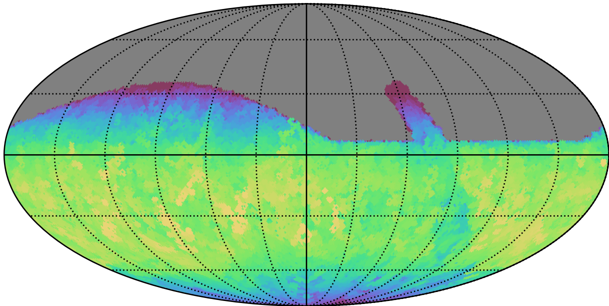
retro_baseline_v2.0_10yrs All sky z band: Max fiveSigmaDepth
