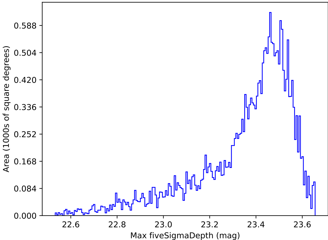
retro_baseline_v2.0_10yrs All sky z band: Max fiveSigmaDepth
