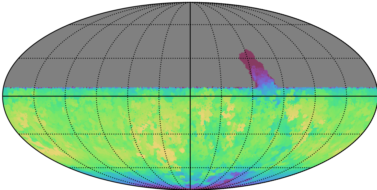
retro_baseline_v2.0_10yrs All sky y band: Max fiveSigmaDepth
