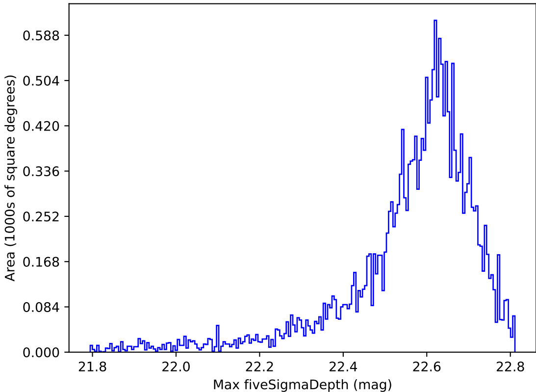
retro_baseline_v2.0_10yrs All sky y band: Max fiveSigmaDepth
