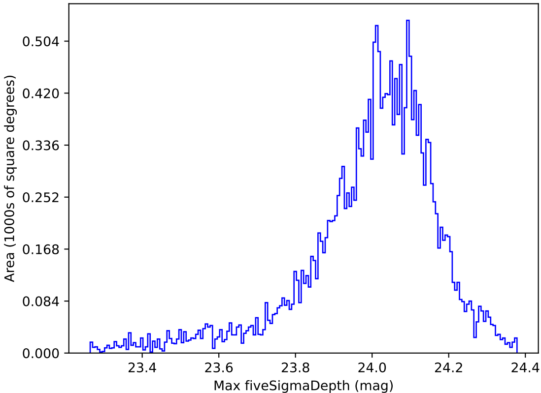
retro_baseline_v2.0_10yrs All sky u band: Max fiveSigmaDepth
