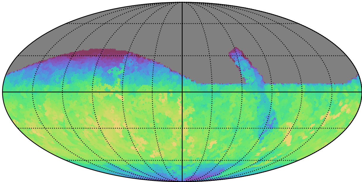
retro_baseline_v2.0_10yrs All sky r band: Max fiveSigmaDepth
