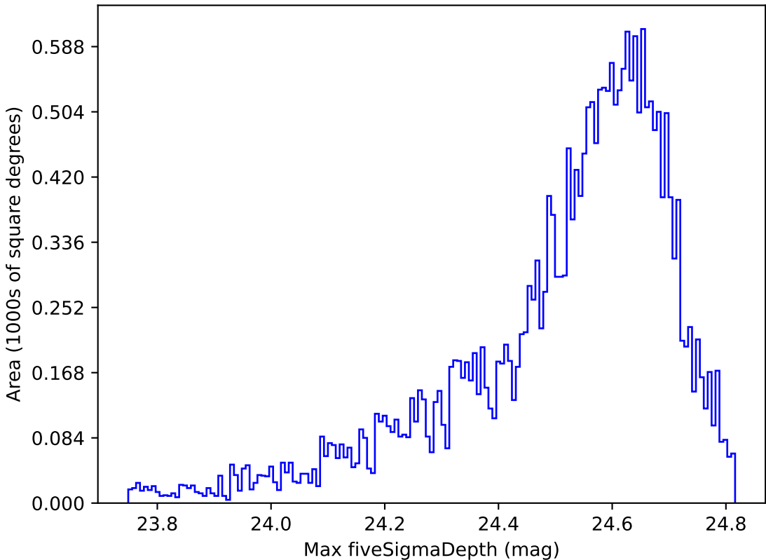
retro_baseline_v2.0_10yrs All sky r band: Max fiveSigmaDepth
