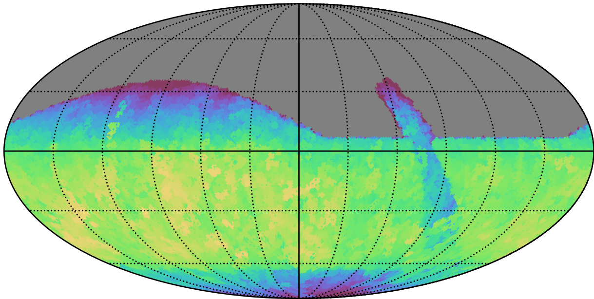
retro_baseline_v2.0_10yrs All sky i band: Max fiveSigmaDepth
