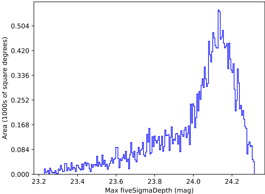
retro_baseline_v2.0_10yrs All sky i band: Max fiveSigmaDepth
