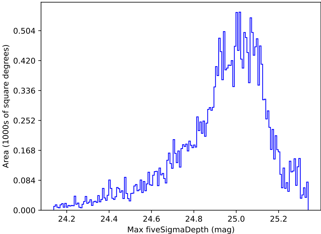
retro_baseline_v2.0_10yrs All sky g band: Max fiveSigmaDepth
