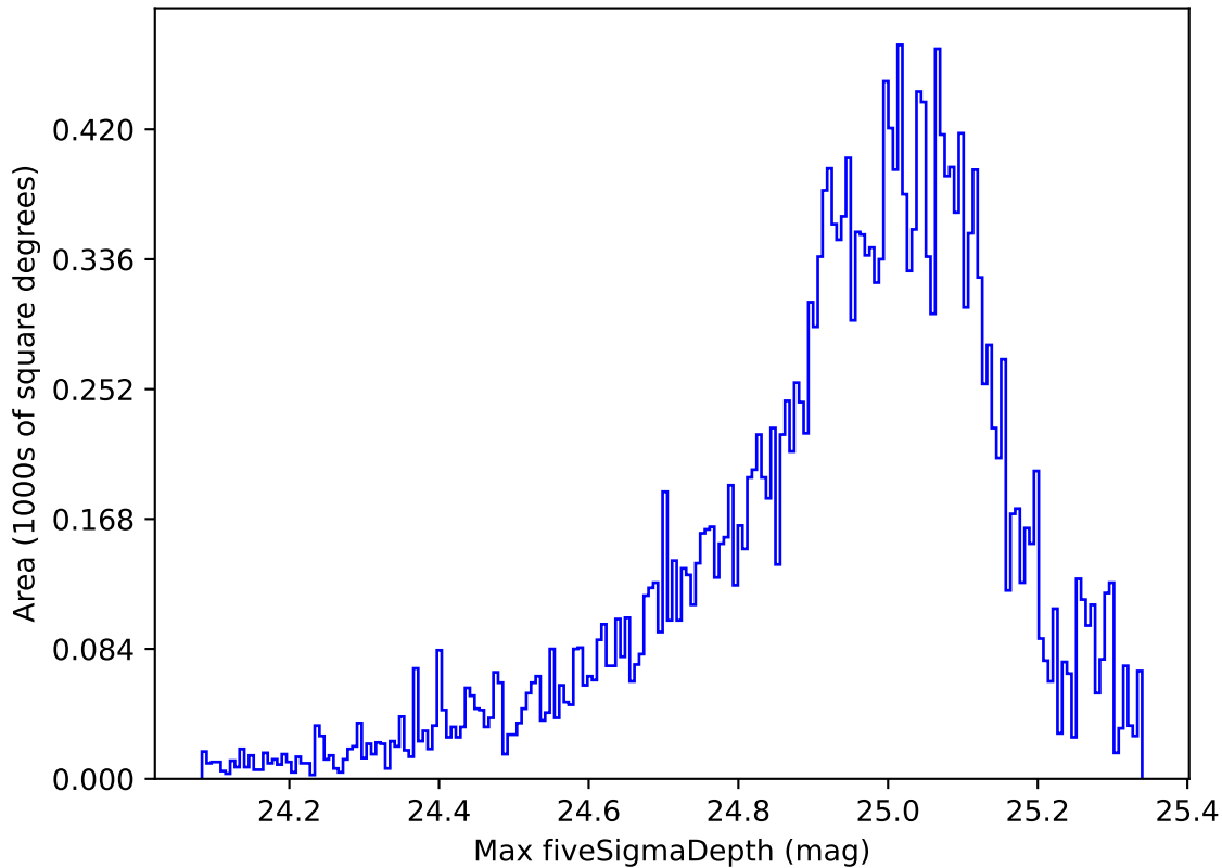
retro_baseline_v2.0_10yrs All sky all bands: Max fiveSigmaDepth
