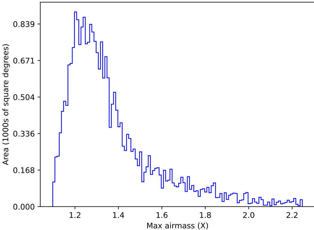
retro_baseline_v2.0_10yrs Yr 1 z band: Max airmass
