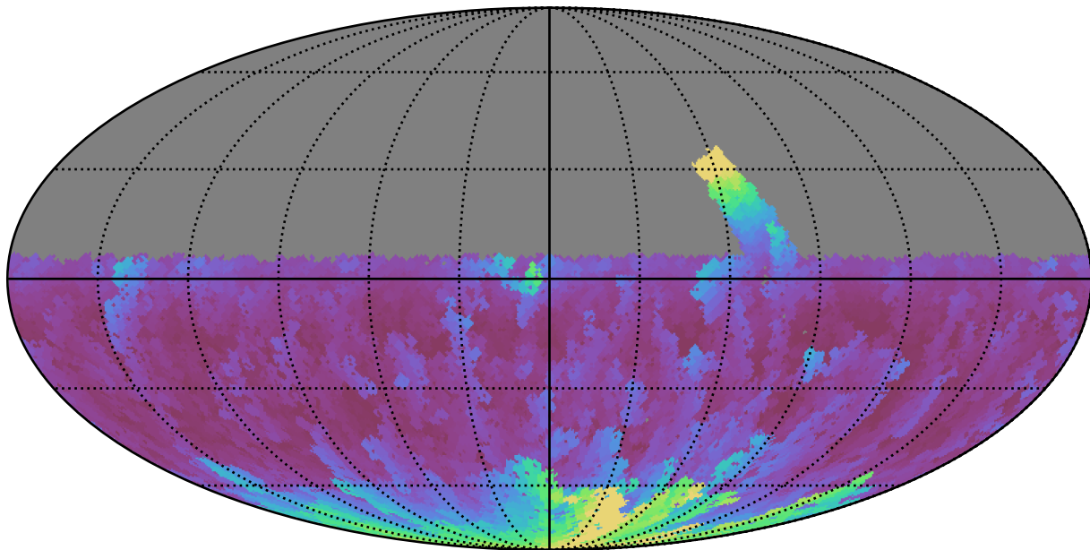
retro_baseline_v2.0_10yrs Yr 1 u band: Max airmass
