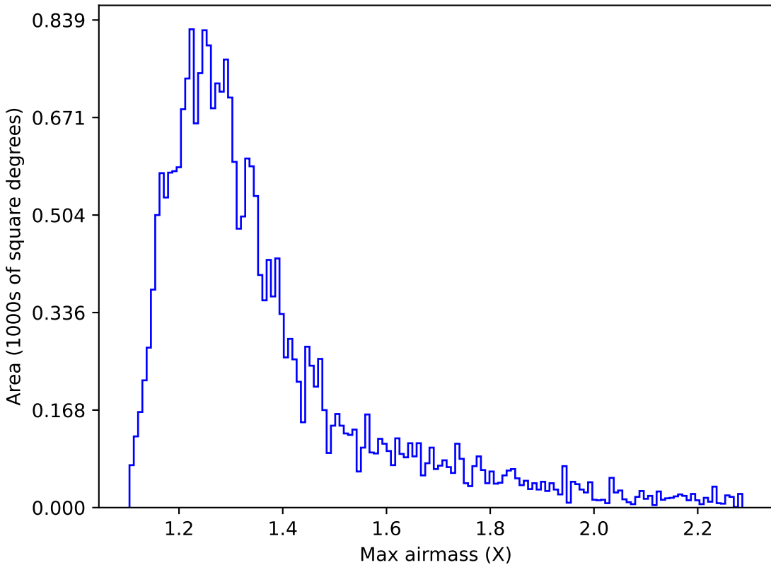
retro_baseline_v2.0_10yrs Yr 1 i band: Max airmass
