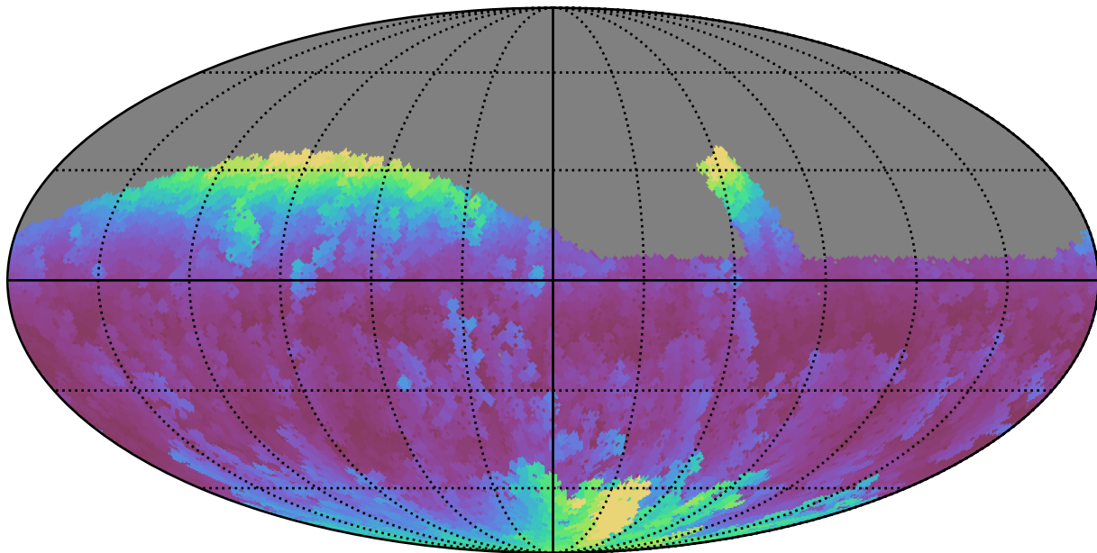
retro_baseline_v2.0_10yrs Yr 1 g band: Max airmass
